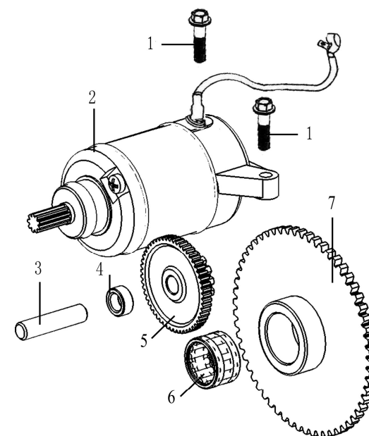
电启动机构 ELECTRIC STARTING MECHANISM
