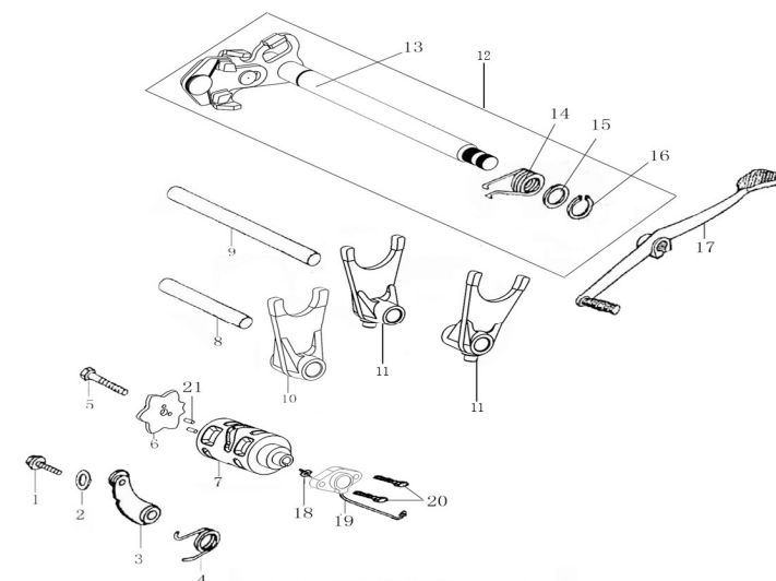
变速机构 GEARSHIFT MECHANISM
